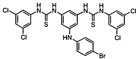
Compound # 11
